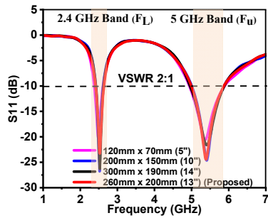
Fig. 8. Effect of varying size of system ground (display screen) on the performance of the presented antenna
