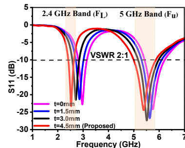
Fig. 6. Effect of varying 't' on performance of the presented antenna
