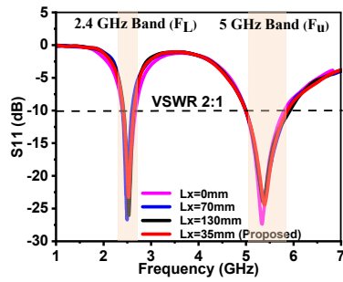
Fig. 7. Effect of varying 'L x ' on performance of the presented antenna
