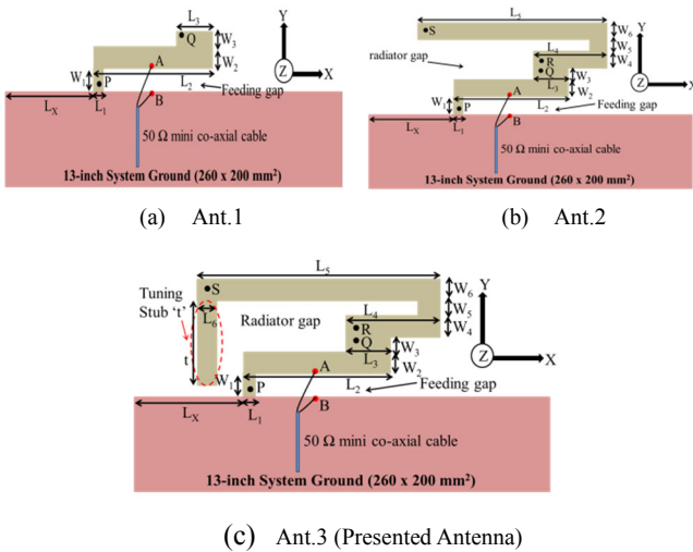
Fig. 2. Complete design process of the presented antenna
