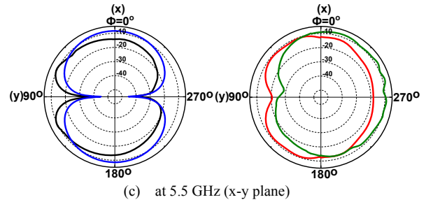
Fig. 11. Simulated and measured radiation patterns in x-y plane
