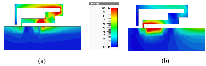
Fig. 5. Simulated surface current (A/m) distribution (a) at 2.45GHz and (b) 5.55GHz of the presented antenna
