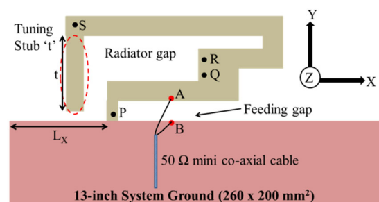
Fig. 1. Schematic geometry of the presented antenna
