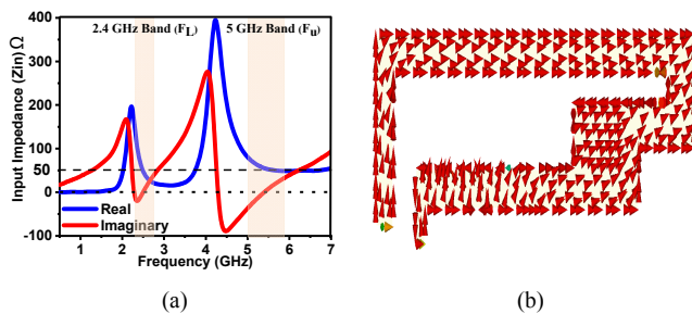
Fig. 4. (a) Input Impedance vs Frequency (b) Current vector distribution of Ant. 3
