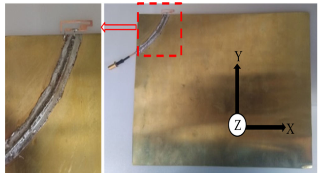
Fig. 9. Fabricated photo of the presented antenna
