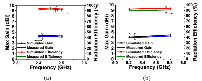
Fig. 12. Simulated and measured gain and efficiency of the presented antenna (a) in F_L band (b) in F_U band
