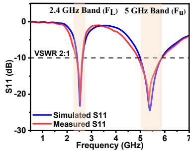
Fig. 10. Comparison of simulated and measured reflection coefficient
