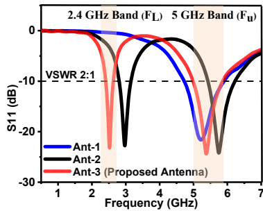
Fig. 3. Simulated reflection coefficient versus frequency for Ant.1, Ant.2 and Ant.3 (Ant. 3 being the presented antenna)
